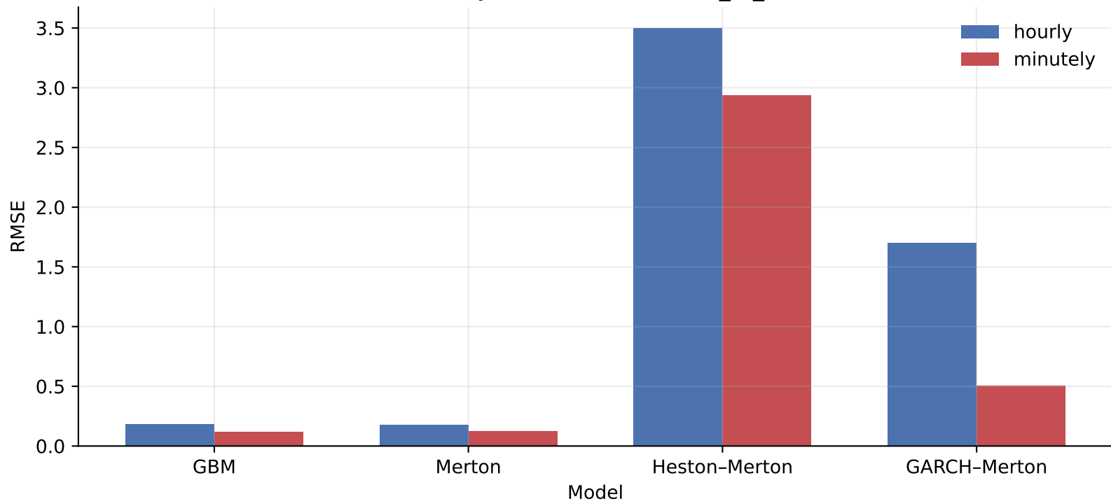
MSFT — RMSE by model · 2023-03-09_to_2023-03-15
