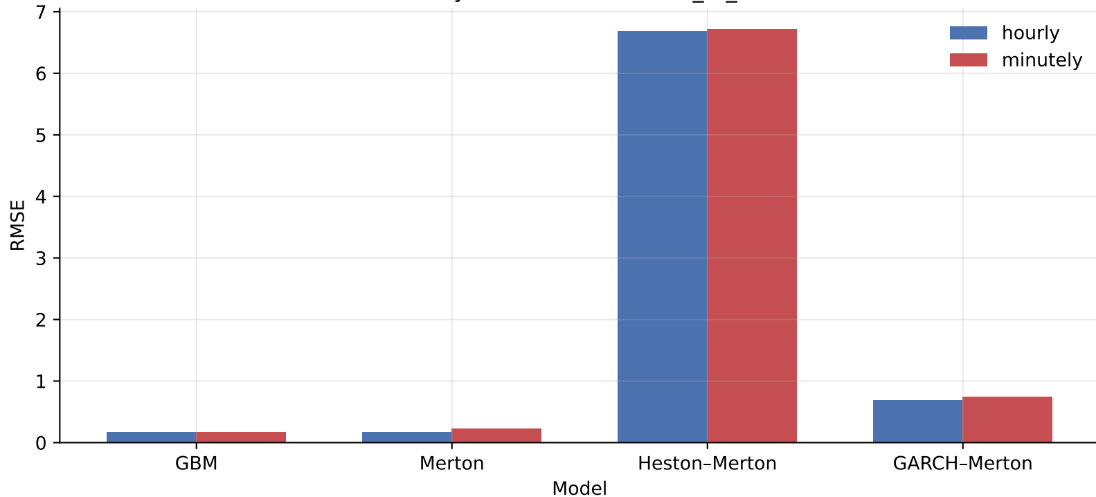
SPY — RMSE by model · 2023-03-09_to_2023-03-15
